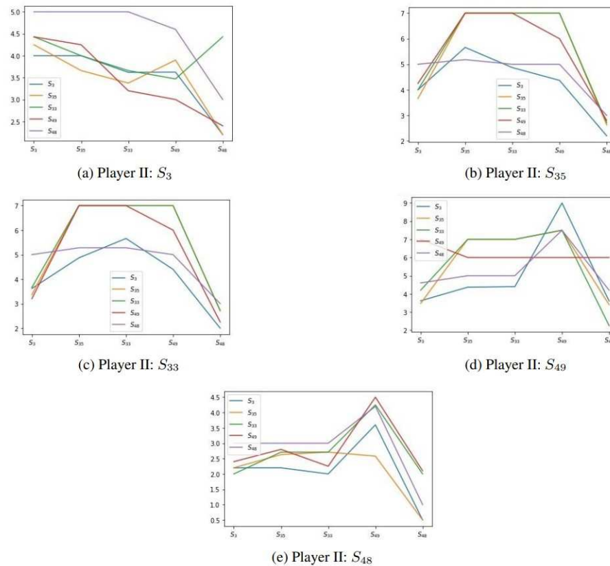
Fig. 2: The payoffs of player I against other strategies
