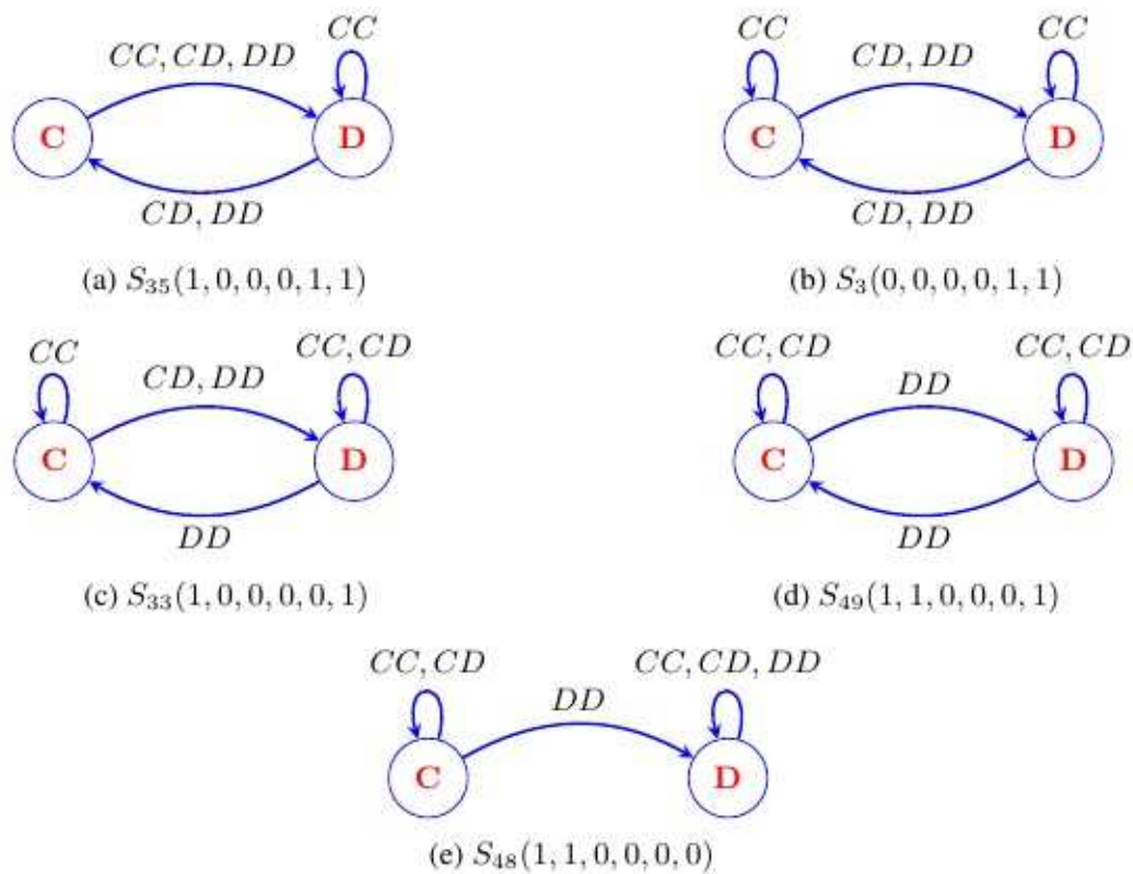
Fig. 1: Automates of WLSL strategies
