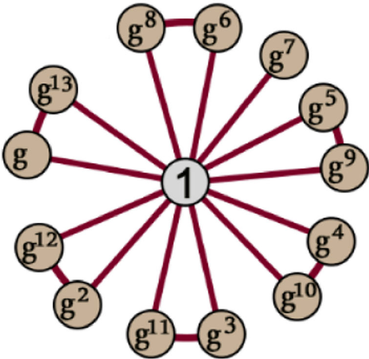
Fig. 1 An identity graph for the cyclic group G = \langle g \mid g^{14} = 1 \rangle
