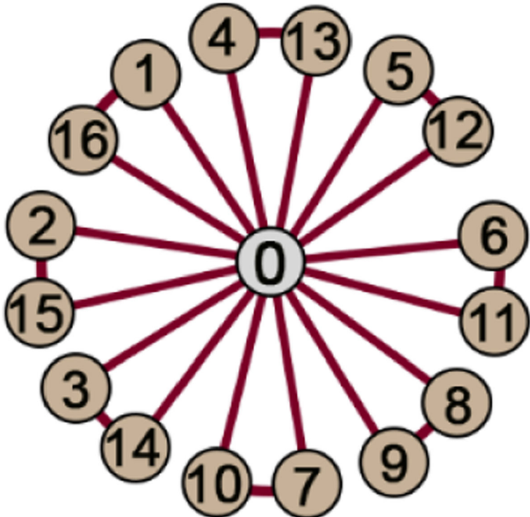
Fig. 2 An identity graph for the Z_{17} = \{0, 1, 2, \dots, 16\} the group under addition modulo 17
