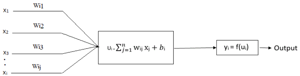
Fig 1. Artificial neural network structure (Cirak and Demirtas 2014)
