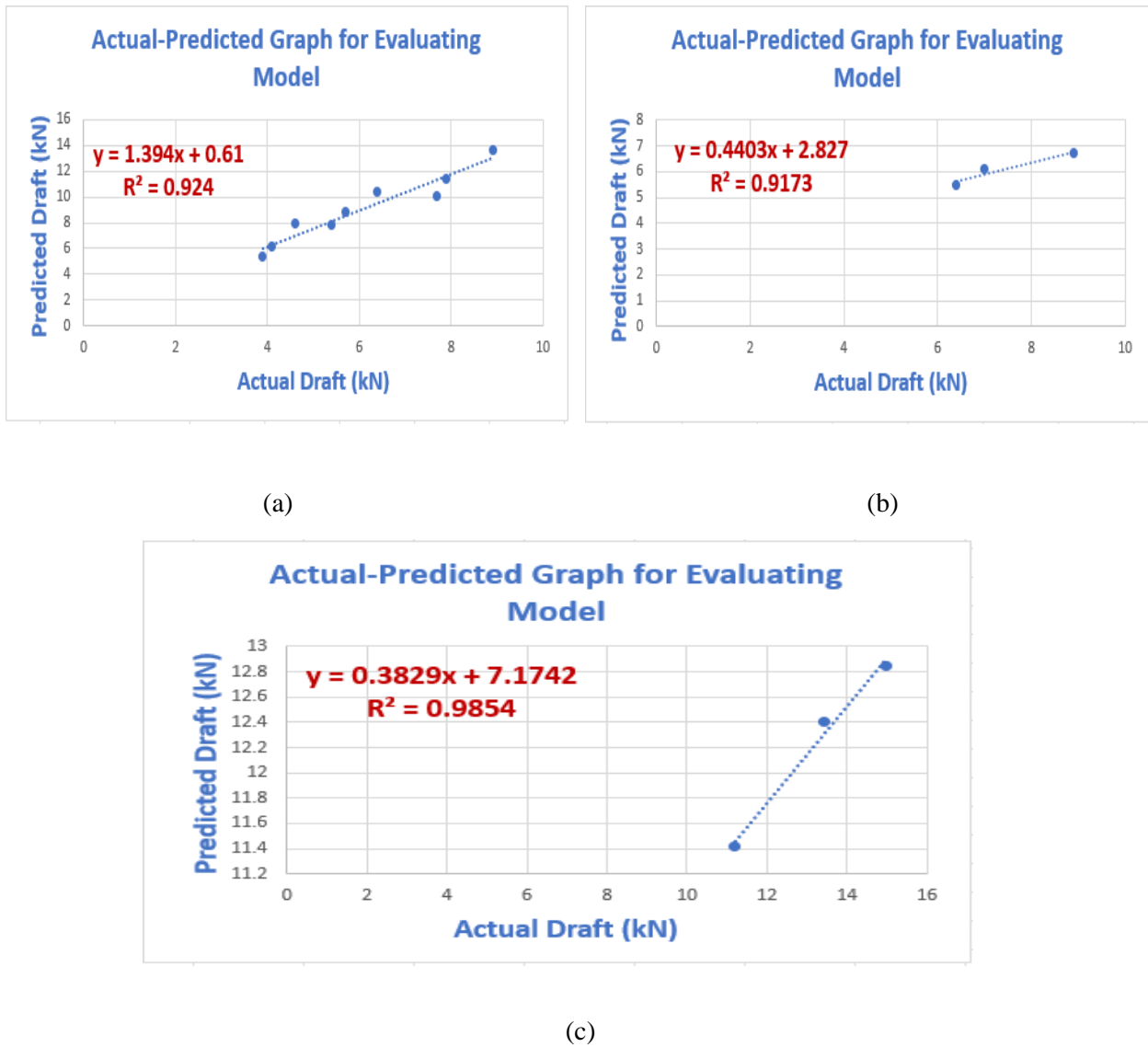
Fig 5. The actual and predicted draft relationship for evaluating the developed ANN-model. (a) moldboard plow, (b) disk plow, (c) chisel plow
