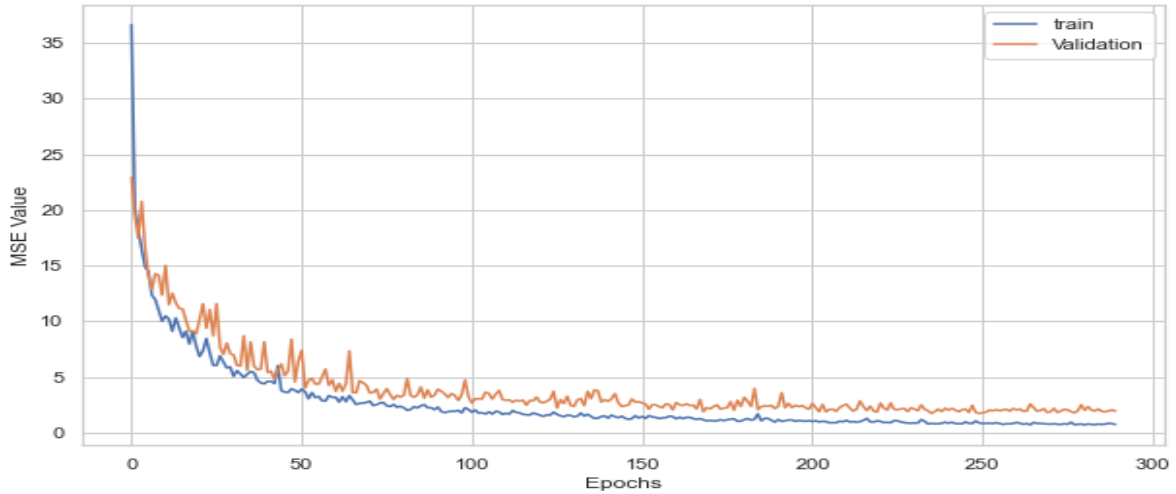
Fig 3. The influence of epochs on the MSE for trained networks
