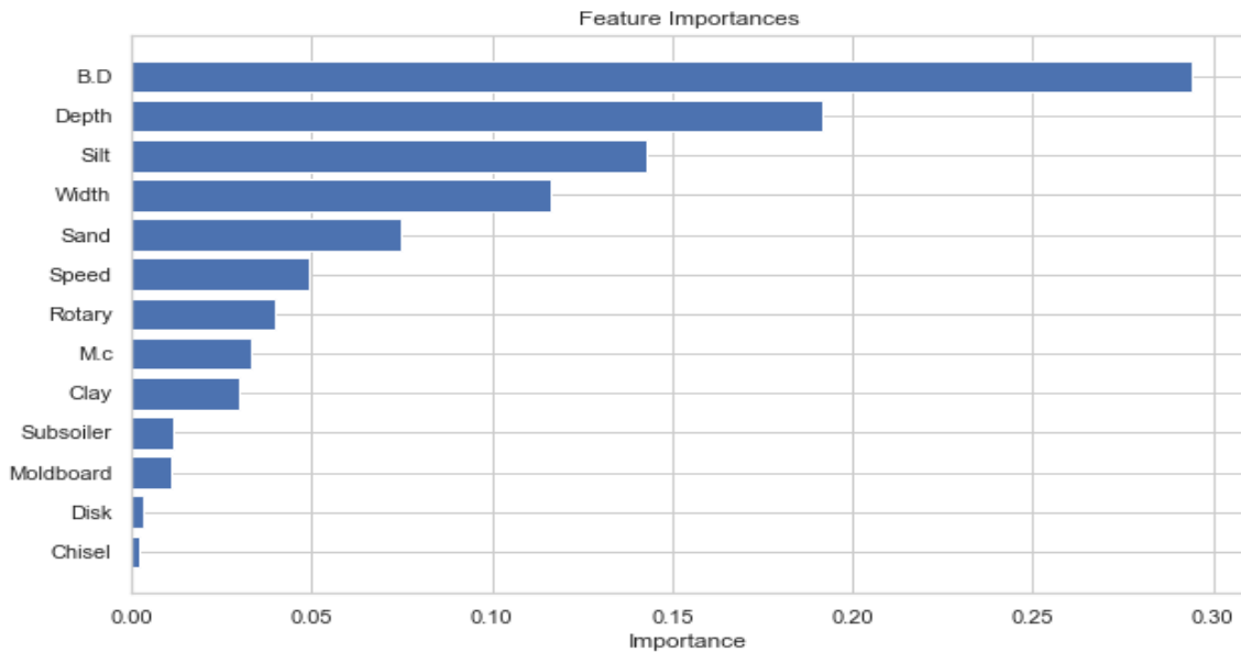
Fig 4. Importance of inputs and their influence on the draft
