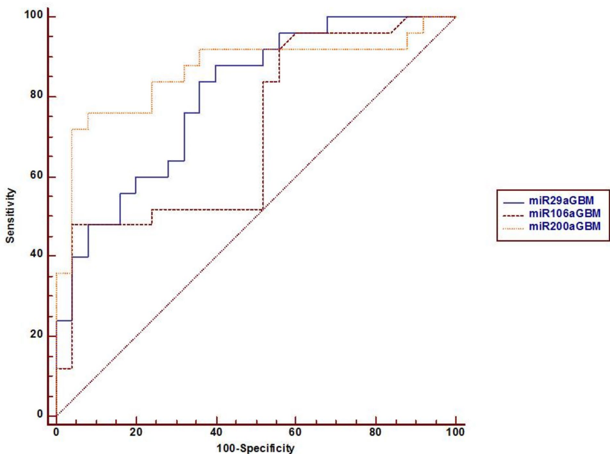
Fig. 2. ROC curve representing the expression of the investigated miRs before and after treatment: miR-29a, AUC = 0.802, 95% CI [0.665–0.901], and SE ± 0.0631 at p = 0.0001 ; miR-106a, AUC = 0.707, 95% CI [0.561 to 0.827], and SE ± 0.0737 at p = 0.0049 ; miR-200a, AUC = 0.864 (95% CI [0.737–0.944], with SE ± 0.0531 at p = 0.0001 ).
