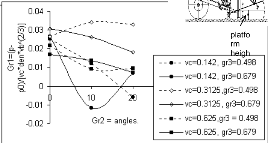
Fig. 11: Relationship between dimensionless groups of conveyor with platform.
