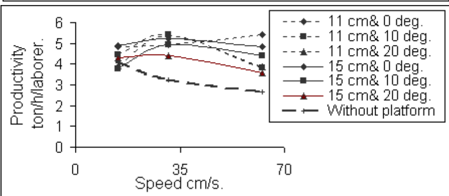
Fig. 12: Productivity of conveyor without and with platform apron at different drive axle speeds, platform heights and angles.
