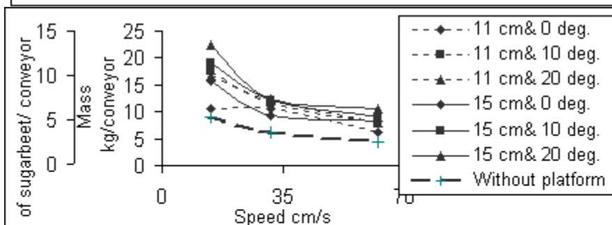
Fig. 14: Mass and No. of sugarbeet on conveyor (4 loaded buckets) at different conveyor speeds without and with platform heights and angles.
