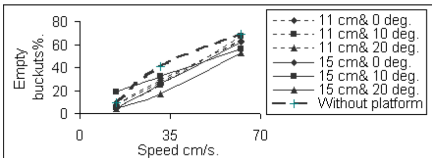
Fig. 13: Missing-buckets percentage of conveyor without and with platform apron at different conveyor speeds, platform heights and angles.
