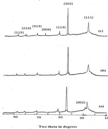
Fig.(1): XRD patterns of CdIn_2Se_4 films with thickness 450 nm at a) 298 K, b) 460 K and c) 580K.
