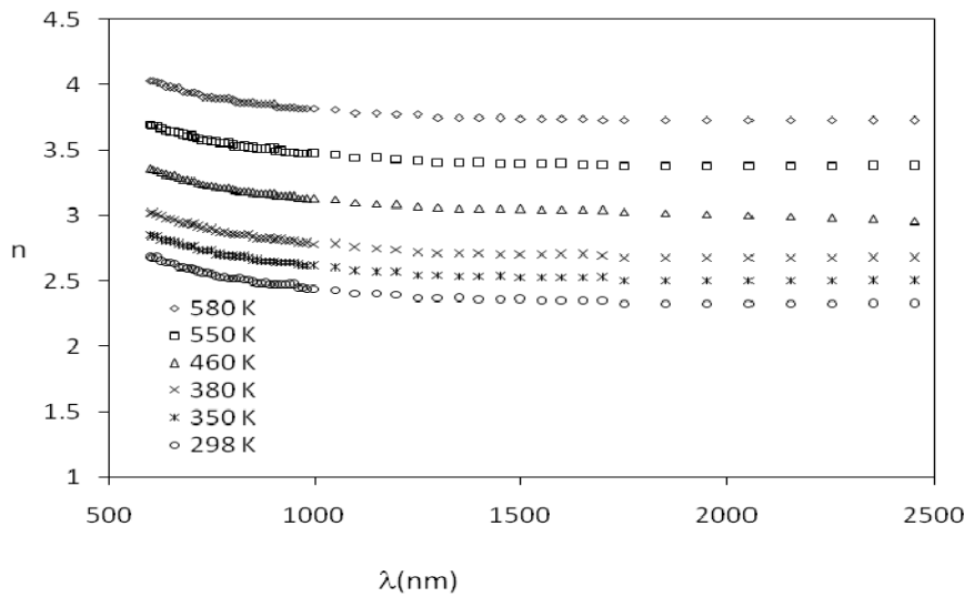
Fig.(6): Plot of refractive index, n versus \lambda for CdIn_2Se_4 thin films with different substrate temperatures
