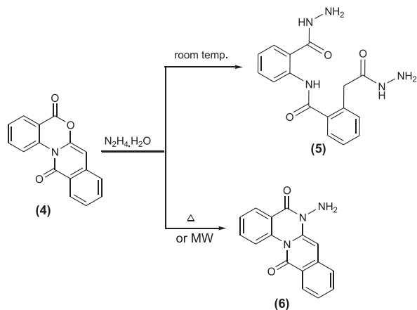
Scheme 3. Synthetic route for the preparation of compounds 5 and 6 .
