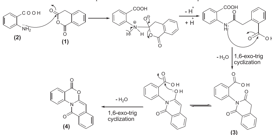
Scheme 2. Proposed mechanism for formation of compound 4 .
