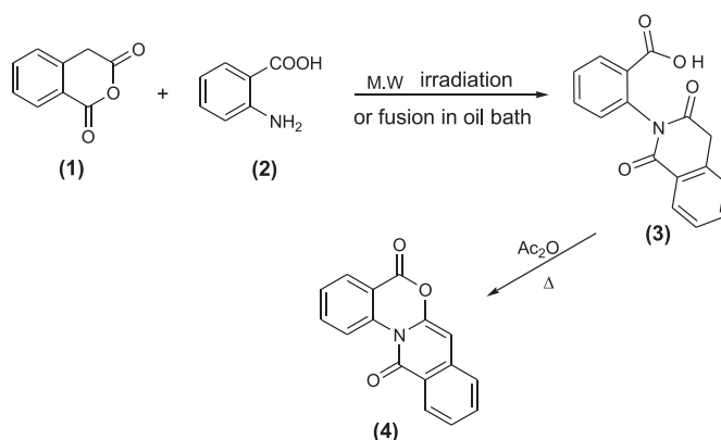
Scheme 1. Synthetic route for the preparation of compounds 3 and 4 .
