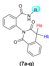
Figure 1. General structure for isoquinolinone derivatives. [Color figure can be viewed at wileyonlinelibrary.com ]
