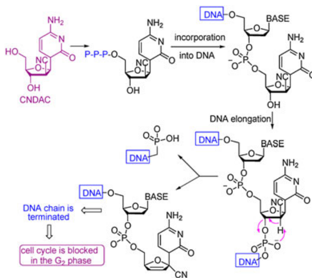
Scheme 6. Mechanism of the antitumor action of CNDAC. [Color figure can be viewed at wileyonlinelibrary.com]
