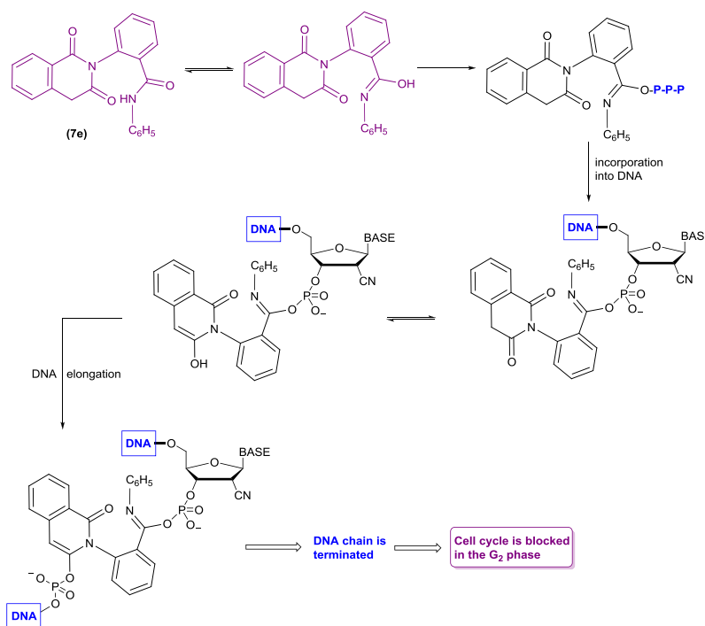
Scheme 7. Mechanism of the antitumor action of compound 7e . [Color figure can be viewed at wileyonlinelibrary.com]
