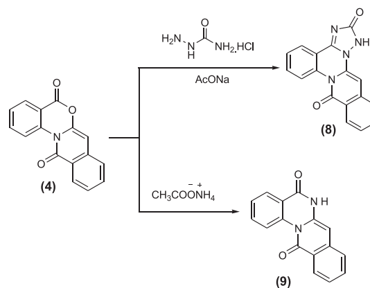
Scheme 5. Synthetic route for the preparation of compounds 8 and 9 .
