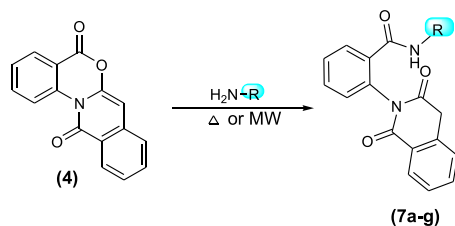
Scheme 4. Synthetic route for the preparation of compounds 7a–g . [Color figure can be viewed at wileyonlinelibrary.com ]
